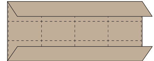
Level-2 Box View from above Outside measurements: W=600 x D=266 x H=168 (3mm cardboard) Inside measurements: W=594 x D=260 x H=162 (3mm cardboard)
